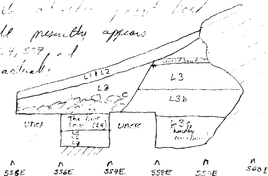
Op 1000 Profile of the SS27N Line
